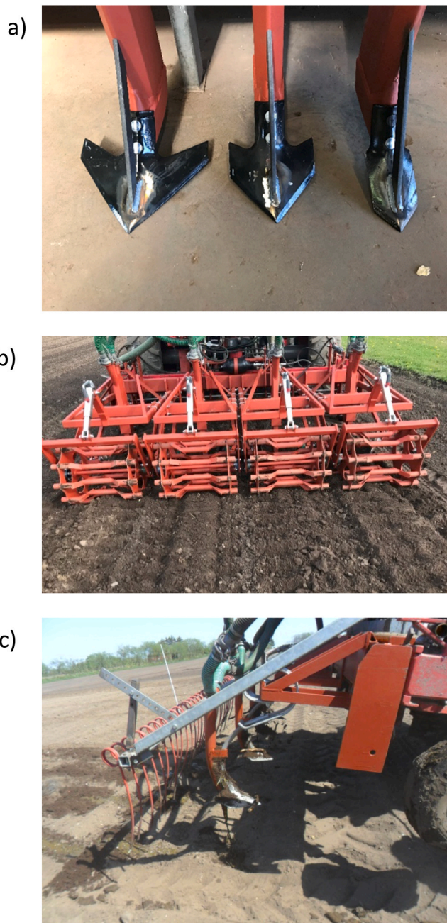
Fig. 1. a) Injection goosefoot tines used in the field trials to placement of slurry with a width of 26 cm (broad), 17 cm (medium) and 8 cm (narrow); b) Rollers installed behind the injection tines; c) Broad goosefoot tine without roller. Photos: Peter Storegård Nielsen and Peter Sørensen, Aarhus University.
